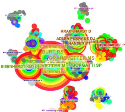
Figure 7 AUTHOR CO-CITATION ANALYSIS
