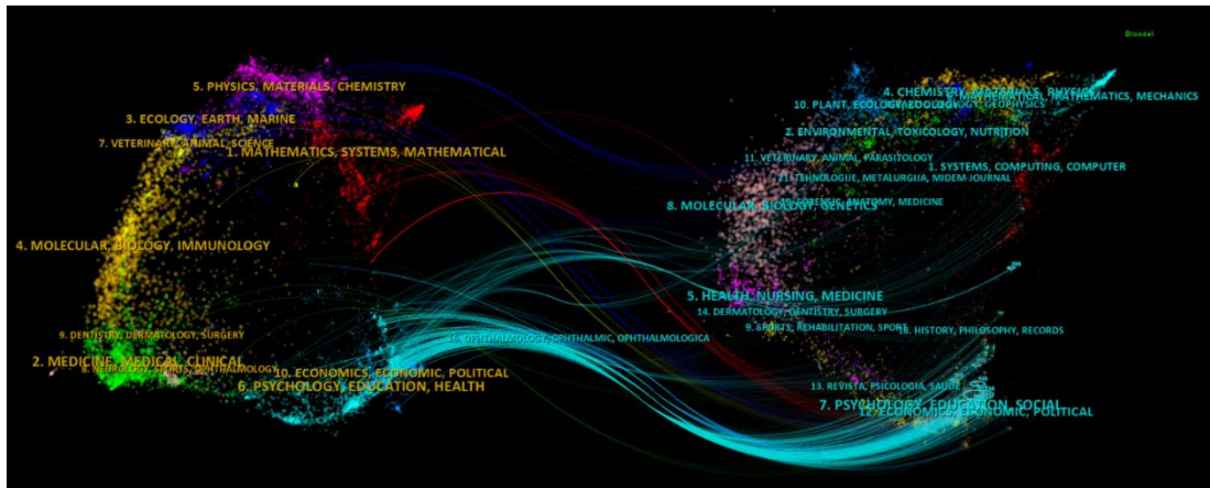
Figure 6. DUAL-MAP OVERLAY OF THE SOCIAL NETWORK THEORY AND SMES
