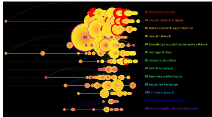
Figure 11 SUMMARY OF THE TOP 13 DOCUMENT CLUSTER LIFETIMES (SOLID LINES)
