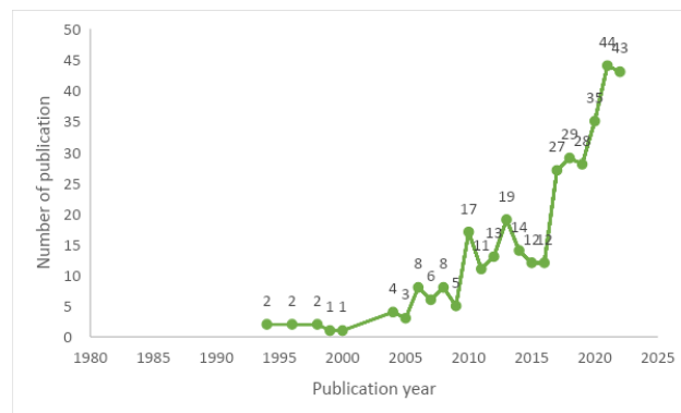
Figure 1 NUMBER OF RESEARCH ARTICLES PUBLISHED ANNUALLY SINCE 1994
