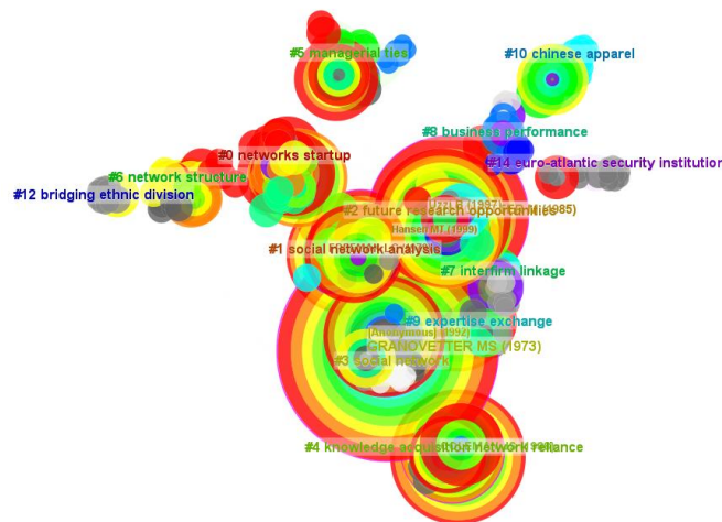
Figure 10 DOCUMENT CO-CITATION ANALYSIS.
