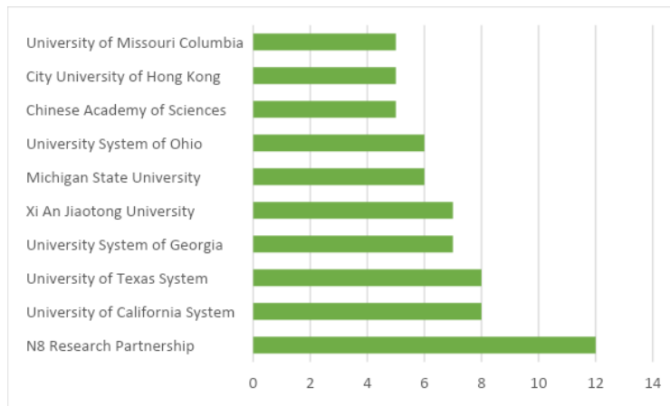
Figure 4. THE NUMBER OF PUBLICATIONS FROM THE TOP 10 INSTITUTIONS
