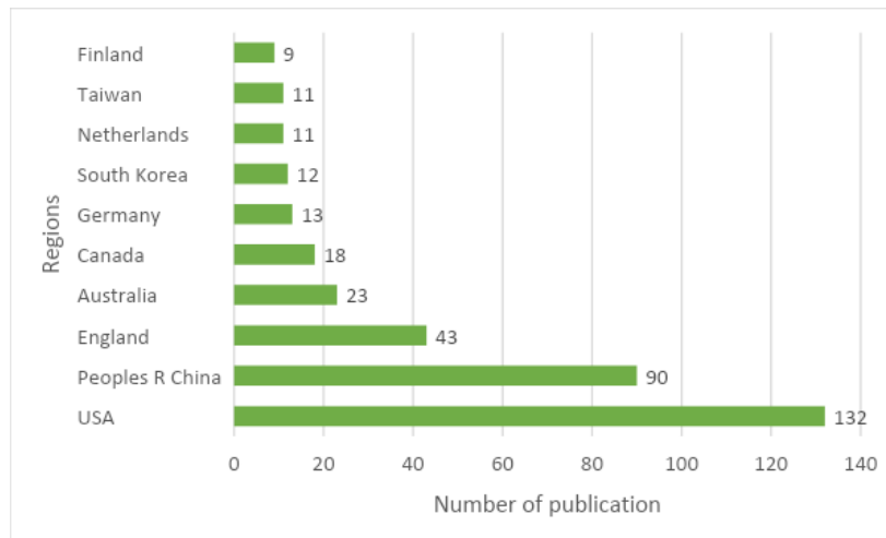
Figure 5 THE NUMBER OF PUBLICATIONS FROM THE TOP 10 COUNTRIES/REGIONS
